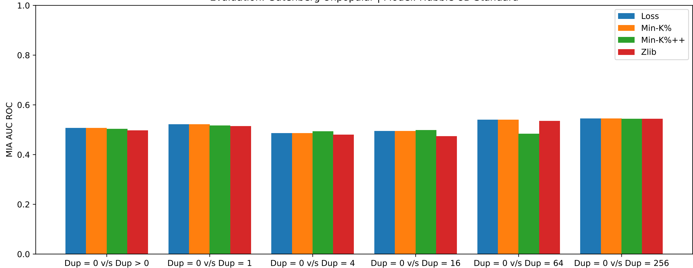
Evaluation: Gutenberg Unpopular | Model: Hubble-8B-Standard
